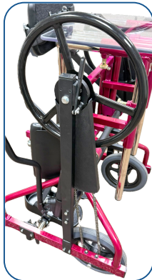
Direct Positive Chain Drive from handrims to lower drive wheels
